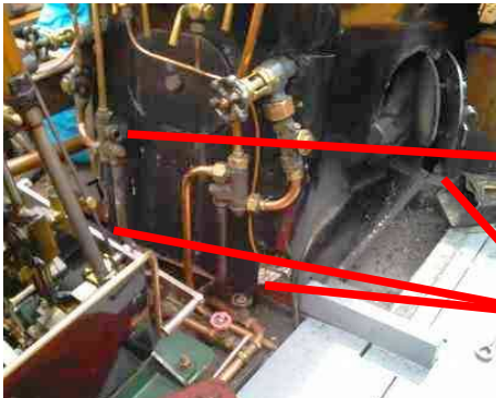
Figure C-2: Washout Plugs
