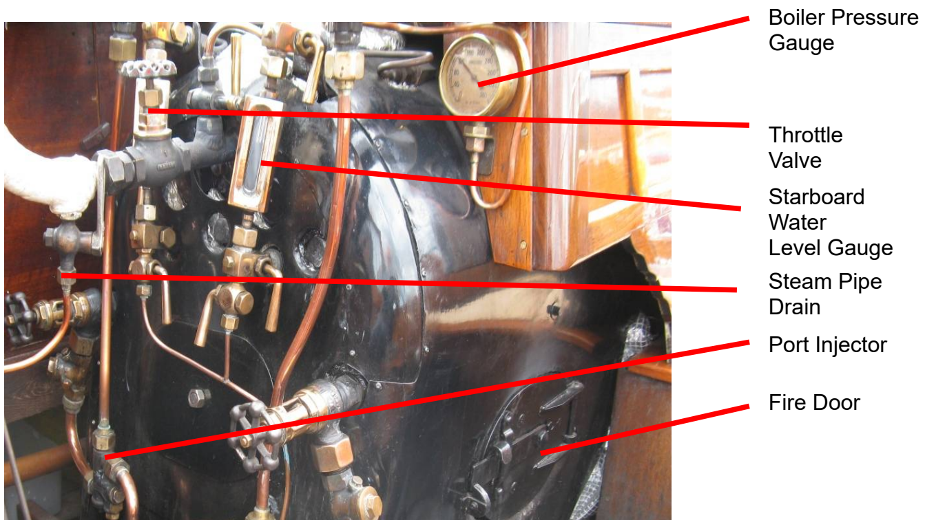
Figure 4-4: The Boiler Face (note that this picture was taken before the injector water control valves were installed – see Figure 4-6 and Figure 4-10)
