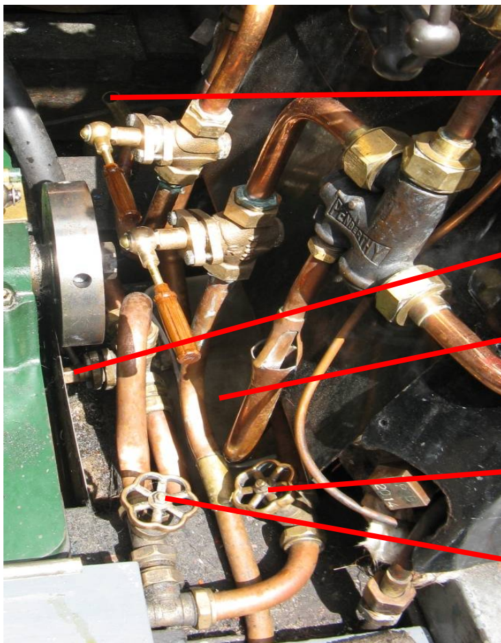
Figure 4-10: Bilge Ejector Valves
